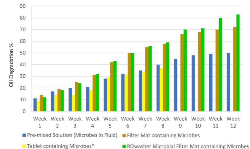
Oil Degradation Rate ROWasher v Competitors
